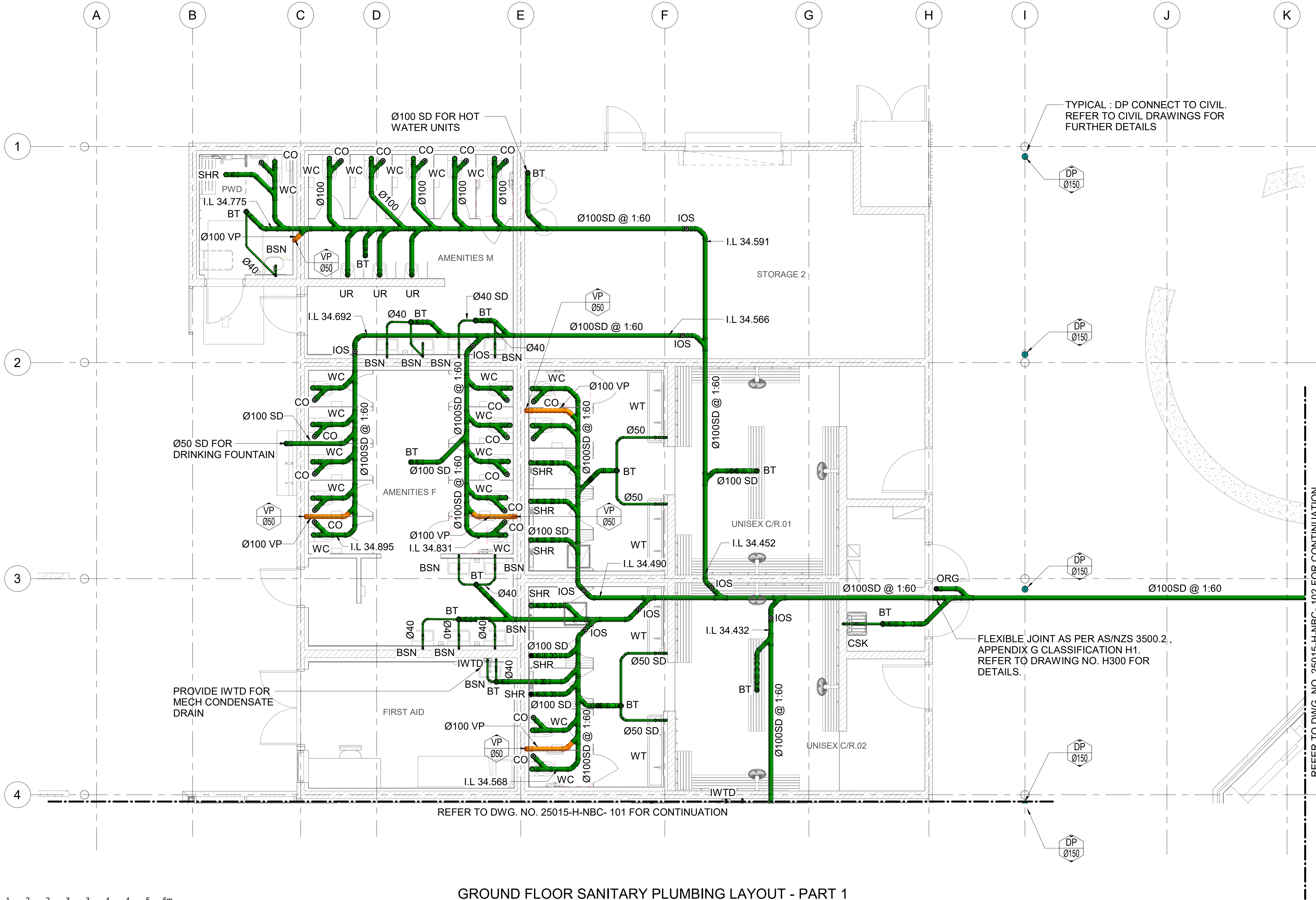
GROUND FLOOR SANITARY PLUMBING LAYOUT - PART 1
